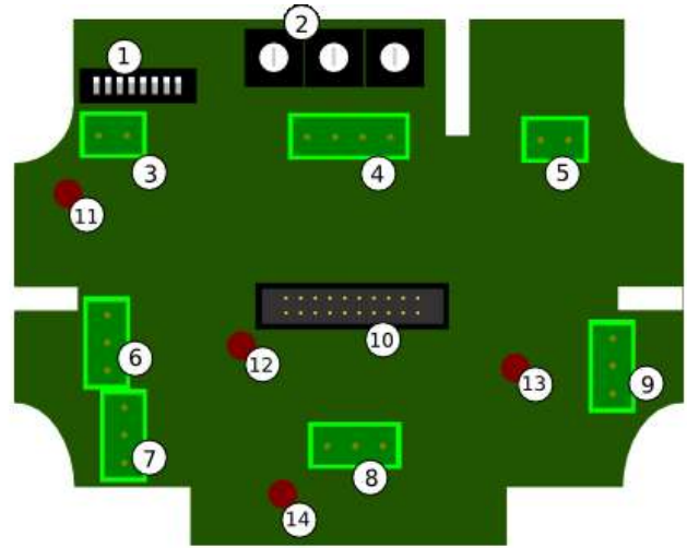
Layout of controller board Mini jumper link located below display connector (not shown)
