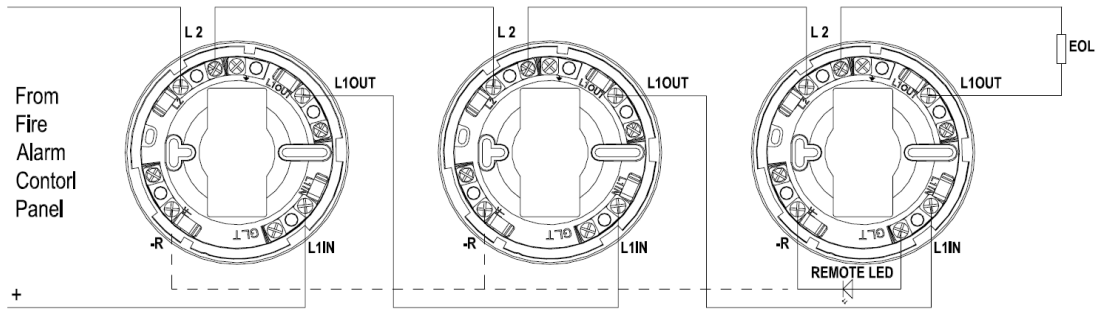
Conventional schematic wiring diagram of detector circuit
